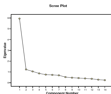
Figure 1: WEMWBS Scree Plot for student samples (n = 348)
