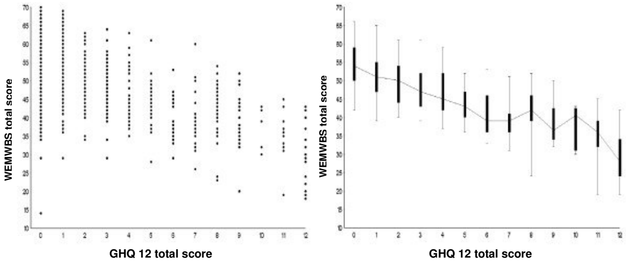
Figure 4: WEMWBS score vs. GHQ 12 score, scatter plot and box and 90% confidence interval whisker plot: population sample
