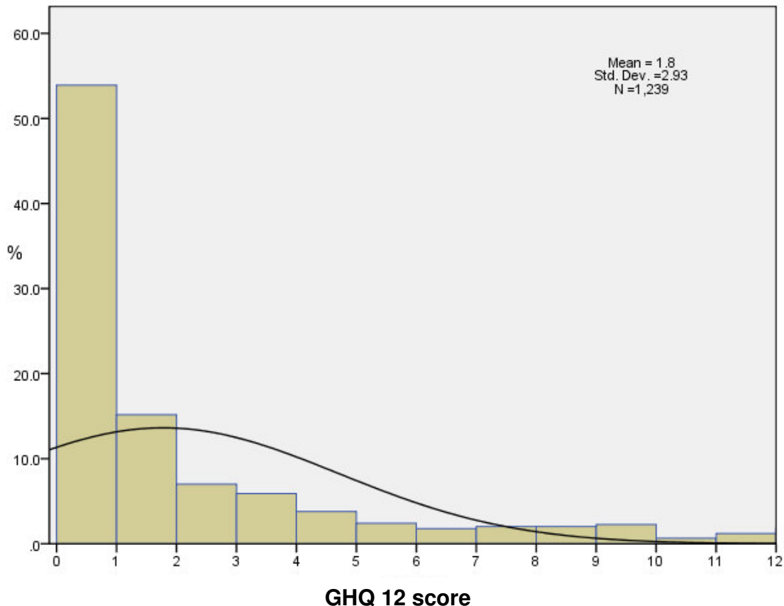
Figure 3: Distribution of GHQ 12 scores for the combined HEPS (wave 12) and Well? 2006 datasets (n = 1,239)
