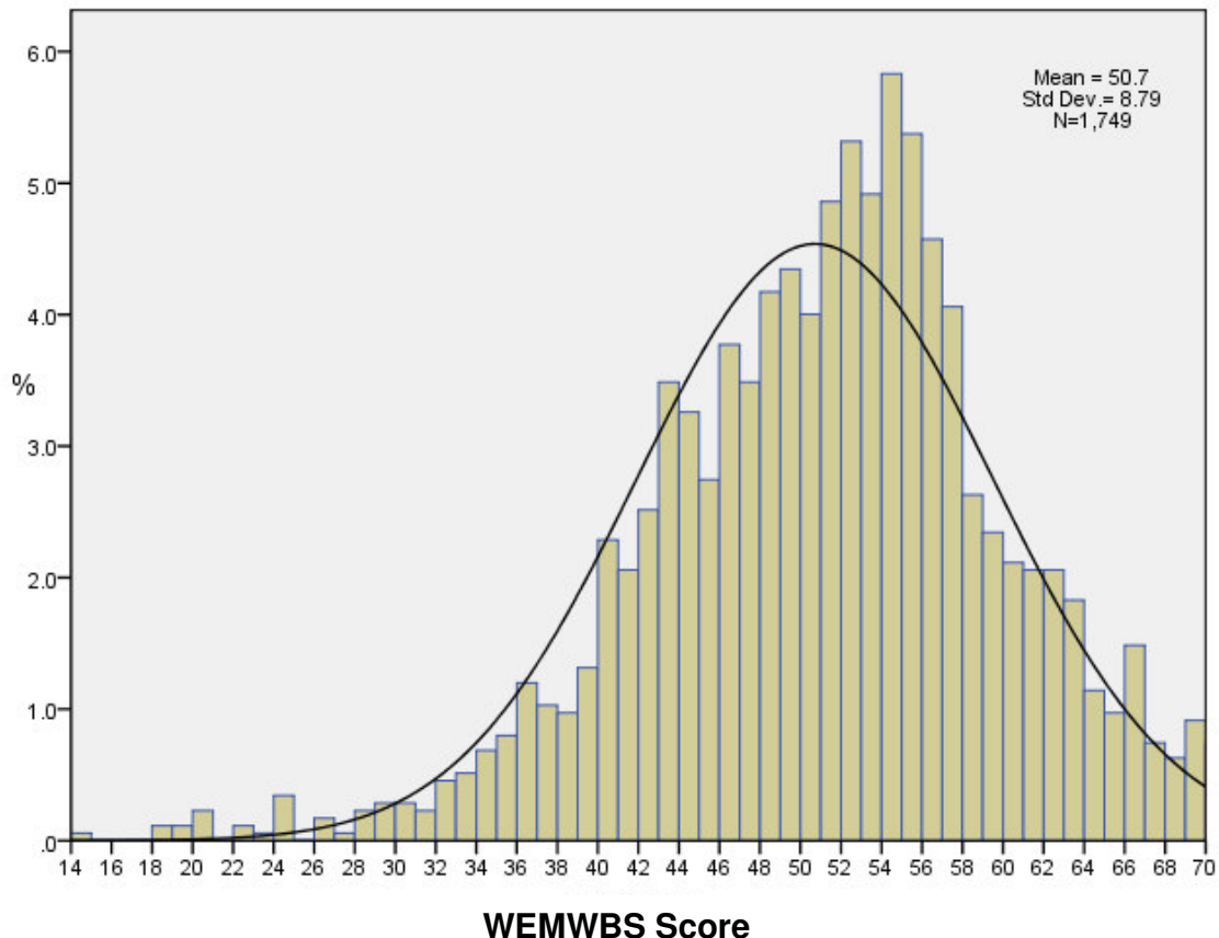
Figure 2: Distribution of WEMWBS scores for the combined HEPS (wave 12) and Well? 2006 datasets (n = 1749)
